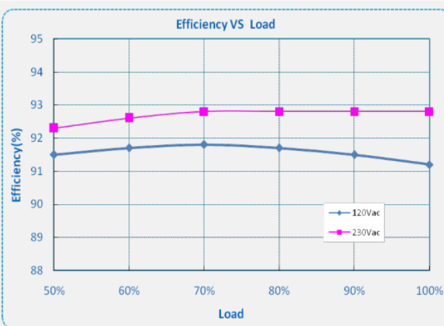
F1-240X056 ( I_o=4.7A )
